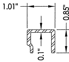
23 REINFORCEMENT 356-A61-B
