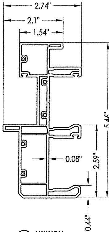
21 MULLION 356-A61
